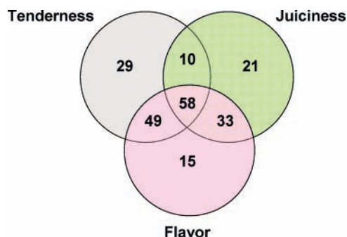
Figure 1. Distribution of the 215 differentially expressed genes in relation to tenderness, juiciness, and flavor.
